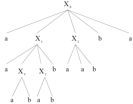
Figure 1. A derivation tree of w
