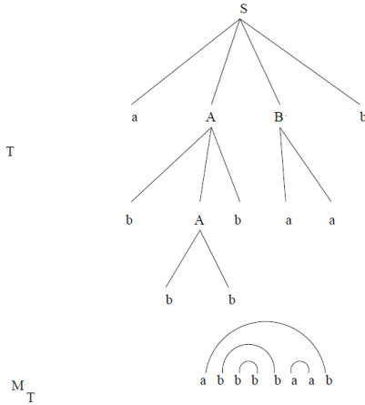
Figure 2. Matching from derivation tree of w
